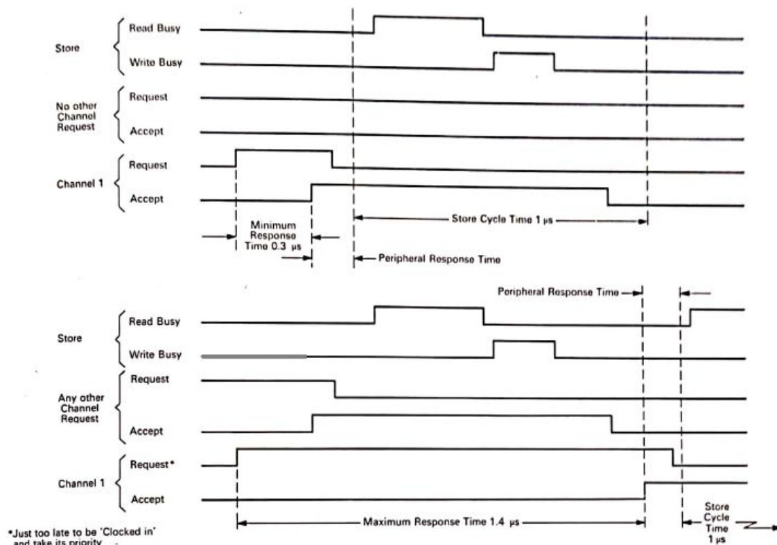
Autonomous Access Response Timing
