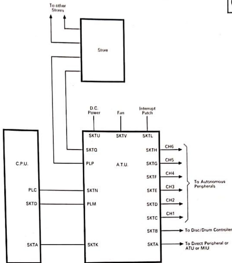
Block Diagram-905 System with A.T.U.
