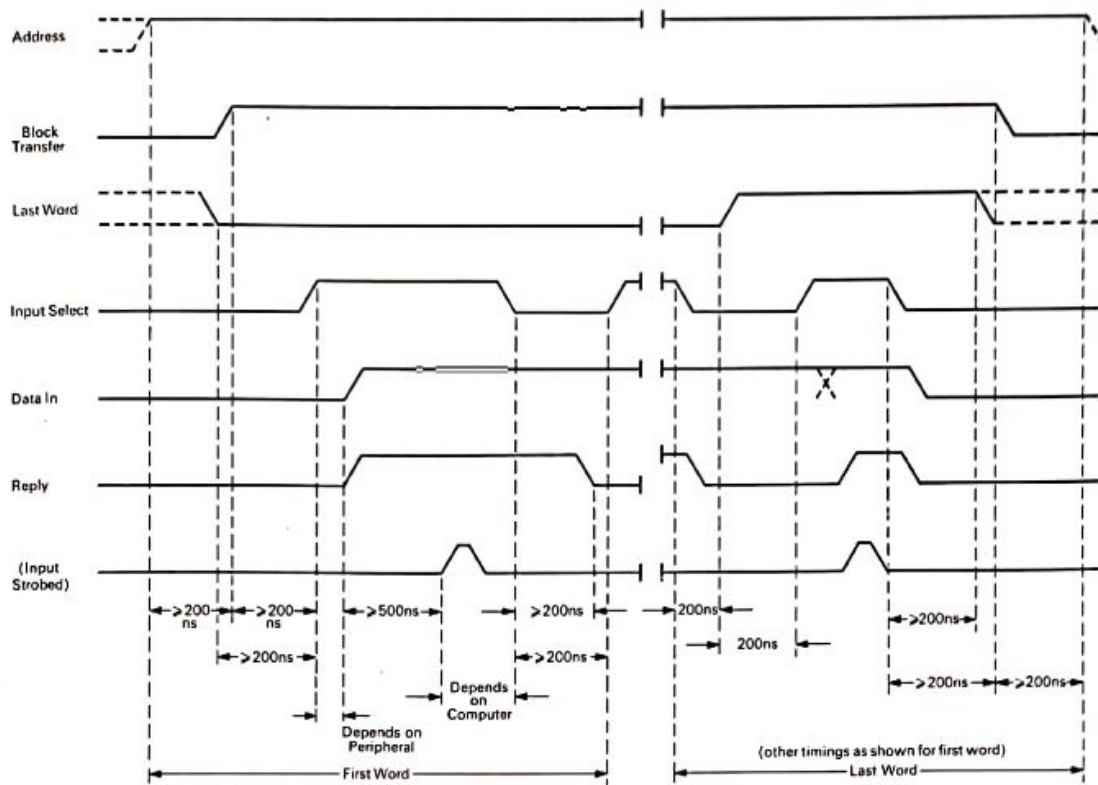
900 Series Interface Block Input Timing
