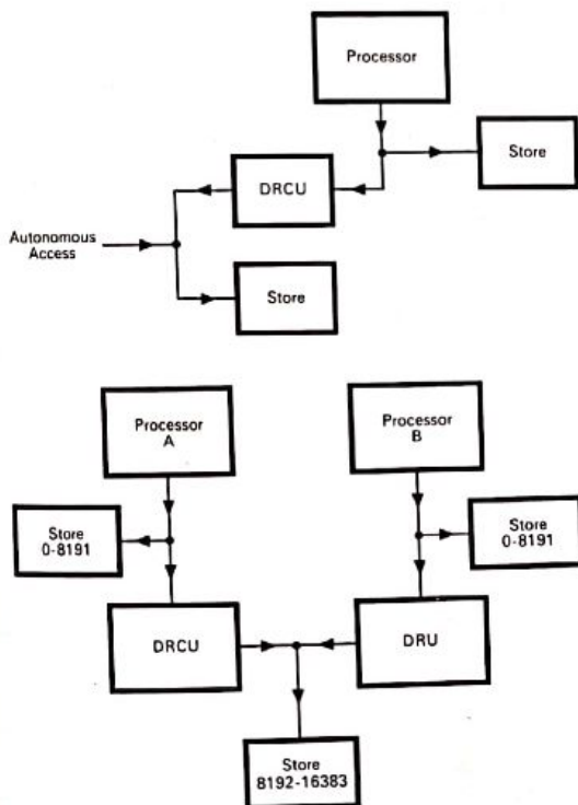
905 Inter-Computer Connections
