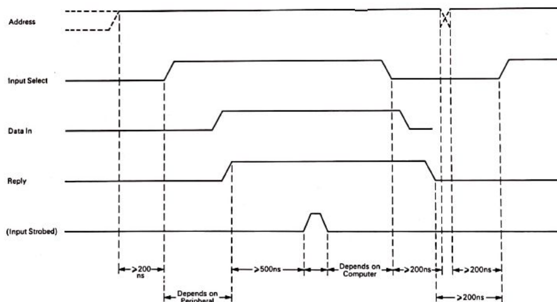
900 Series Interface Single Word Input Timing
