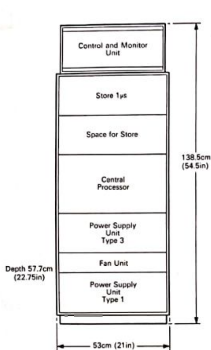
Dimensions, 905 Standard System, 1 \mu s Store
