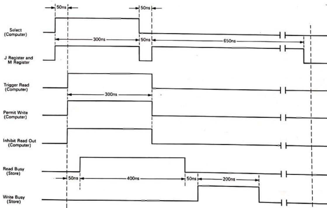
Data Output Timing
