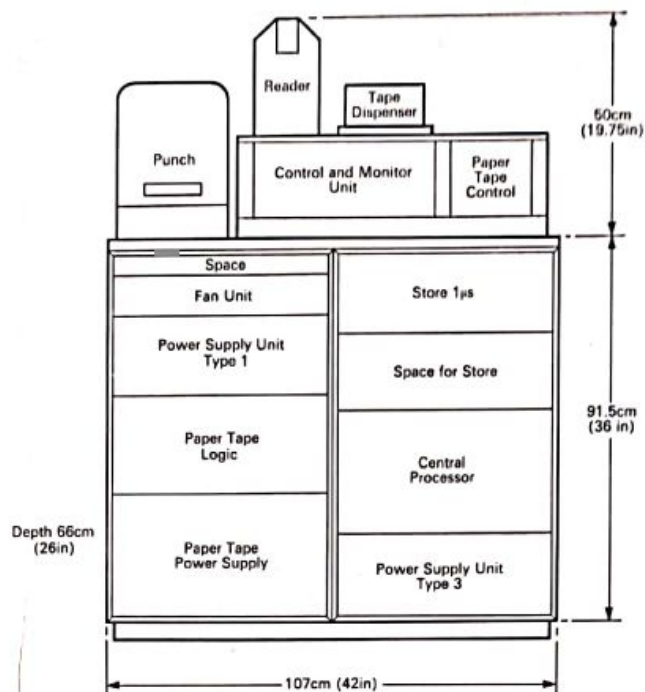
Dimensions, 905 Desk-Mounted System, 1 \mu s Store
