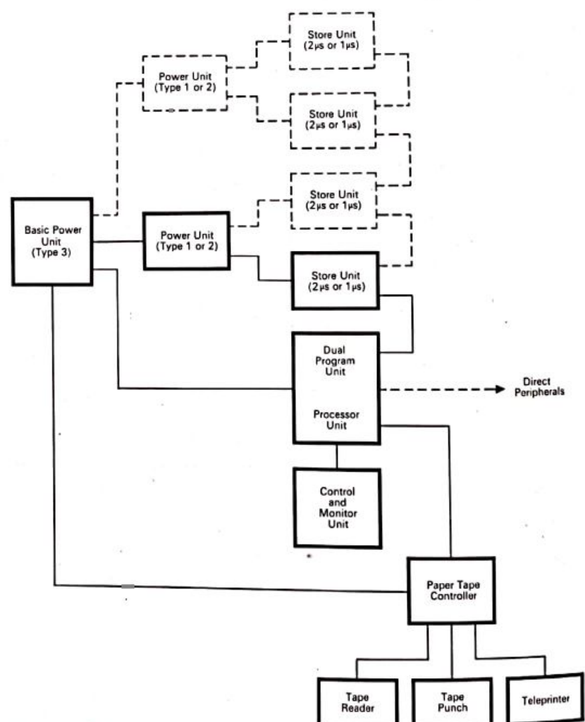
Block Diagram-Extended 905 System
